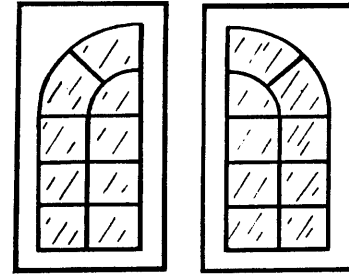
9 LIGHT SPLIT FULL ROUND* (Order as 2 doors 1 left/1 right)
