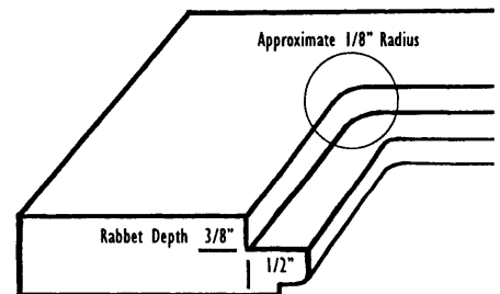
Sample of Standard Rabbit for Optical and Prism Doors
